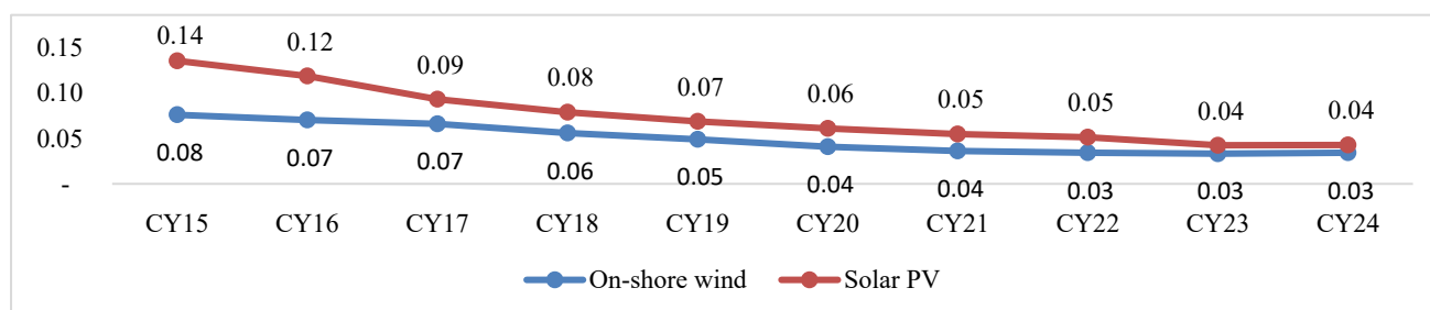
Global weighted average LCOE of wind and solar energy (in $/kW, CY15-CY24)
