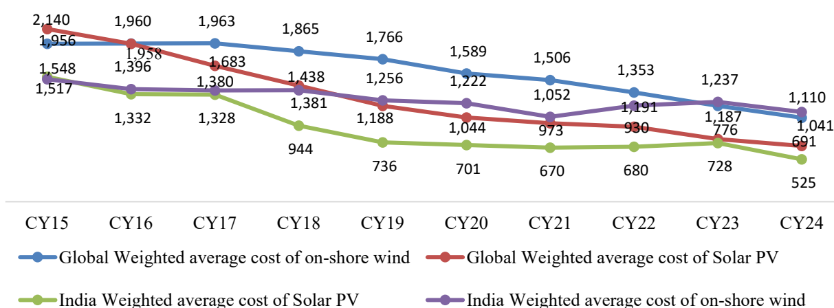
Solar and wind energy installation cost (in $/kW, CY15-CY24)
